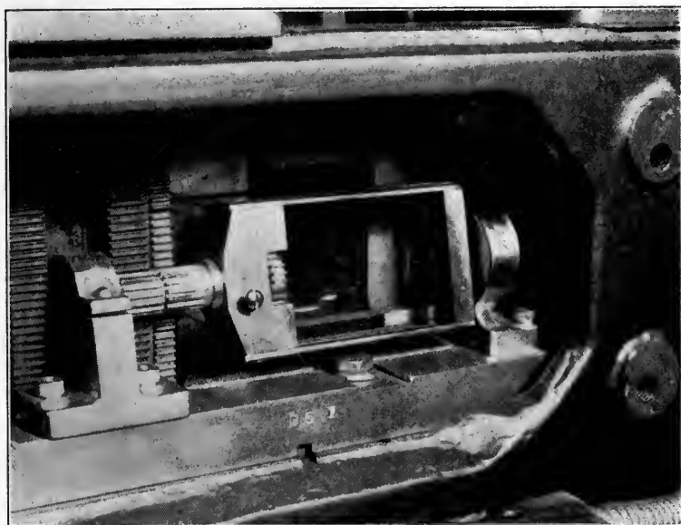
FIG. 3. Close-up of plane-parallel glass plate; note the pinion-gear engaged by the ring-gear and the gear on the slide-carrier.
